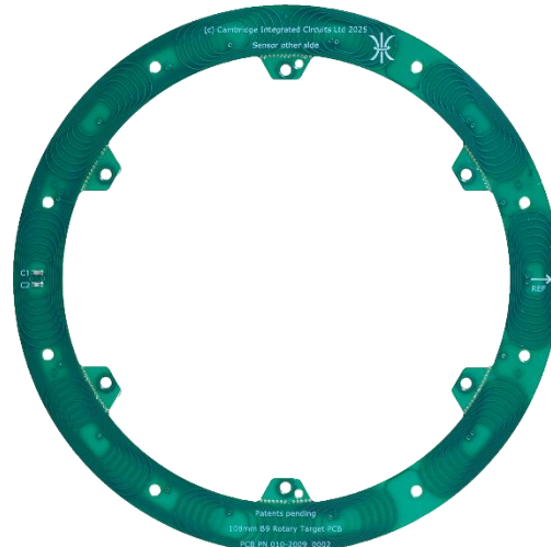
Figure 2 Target Assembly 013-1045, Front
