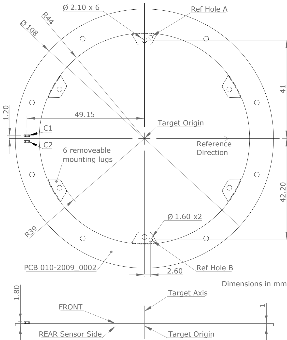
Figure 6 Assembled Target 013-1045
