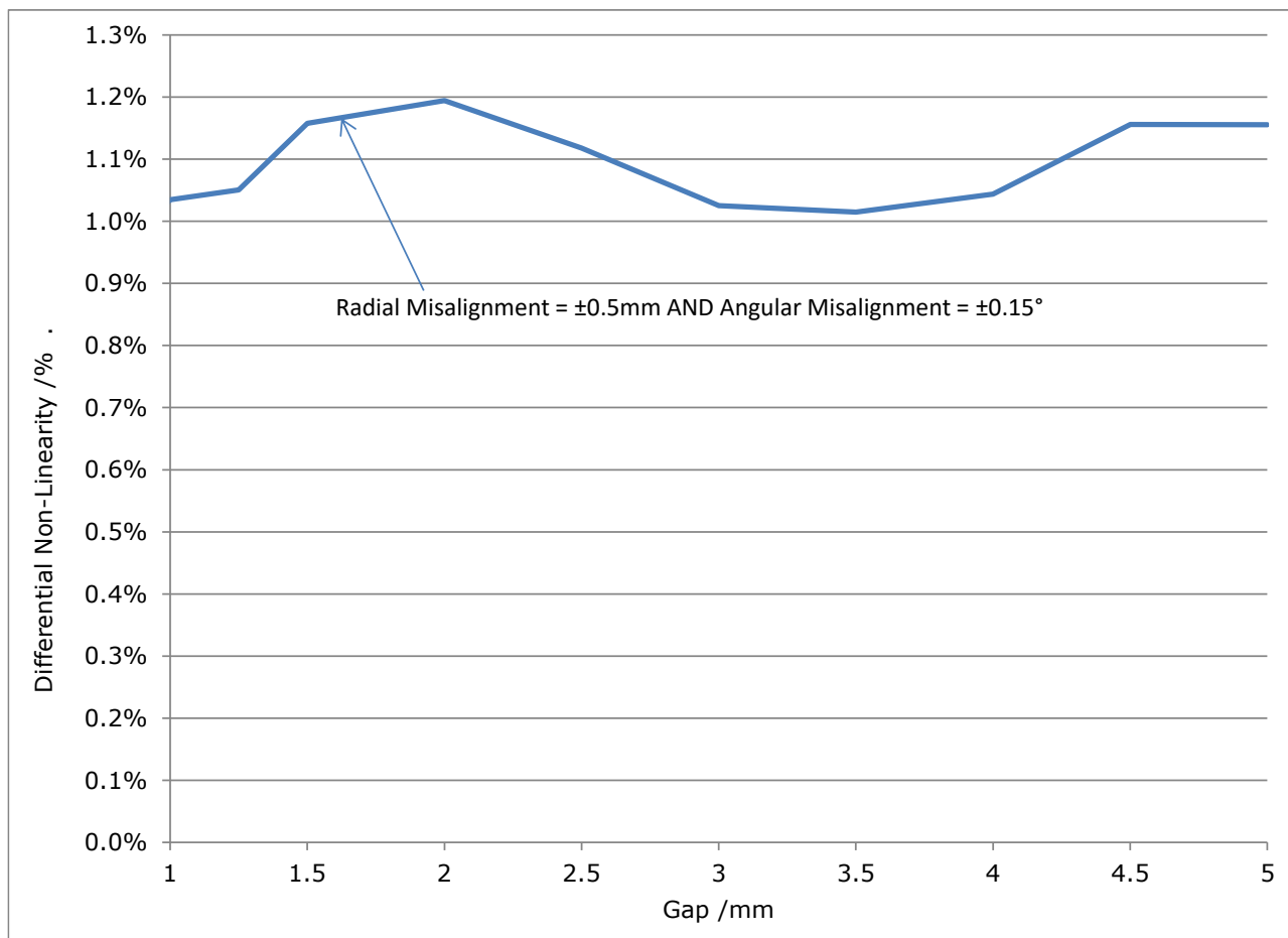
Figure 10 Differential Non-Linearity
