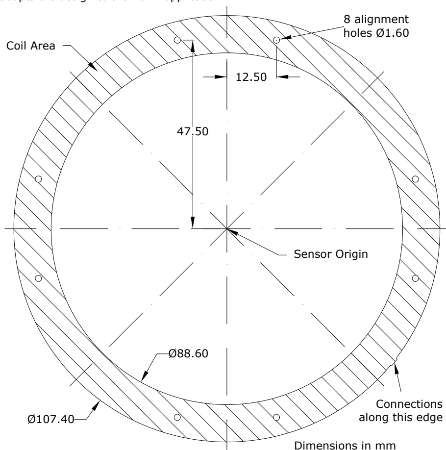
Figure 5 Sensor Coil Area and connections
