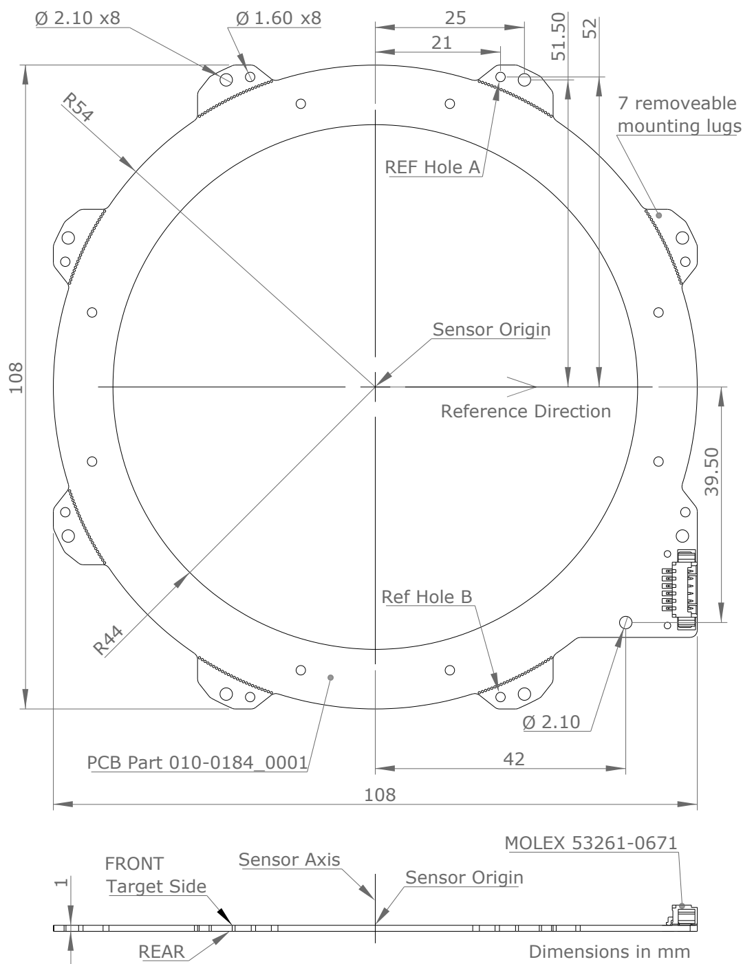
Figure 4 Assembled Sensor 013-0074
