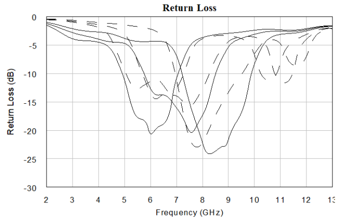
Typical Performance 5.5 to 9.0 GHz
