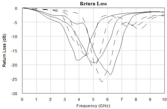
Typical Performance 3.5 to 6.5 GHz
