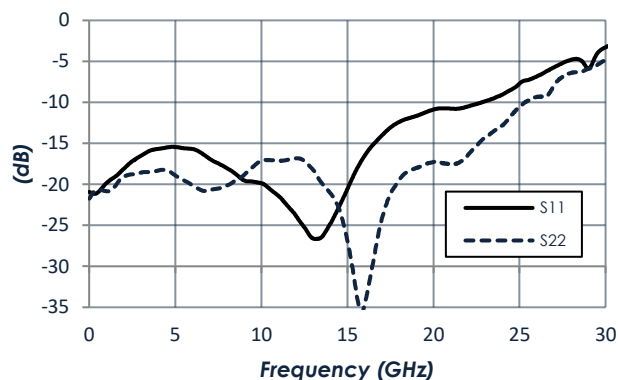
RF2/RF3 Return Loss at +25C
