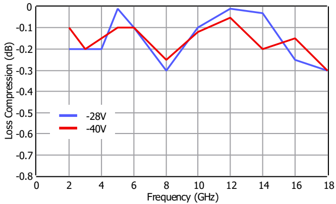
Loss Compression, Pin = 40.5dBm
