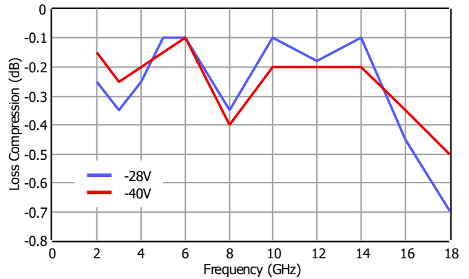
Loss Compression, Pin = 41.5dBm
