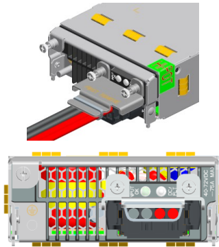
Front View – with input cable retention
