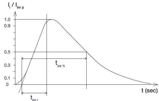
Figure 6. Inrush Current
