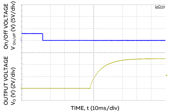
Figure 5. Typical Start-up Using Remote On/Off, negative logic version shown ( V_{in} = 24V or 48V )
