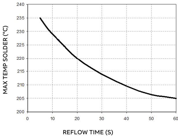
Figure 25. Time Limit Curve Above 205°C for Tin/Lead (Sn/Pb) process
