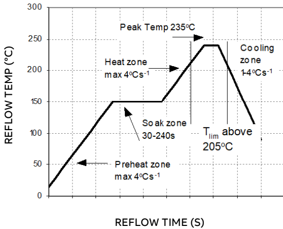
Figure 24. Reflow Profile for Tin/Lead (Sn/Pb) process.
