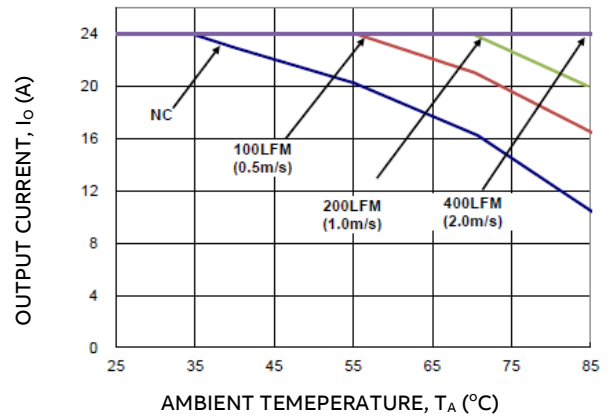
Figure 18. Output Current Derating for the Open Frame Module; Airflow in the Transverse Direction from V_{out(-)} to V_{out(+)} ; V_{IN} = 24V, V_O = 5V
