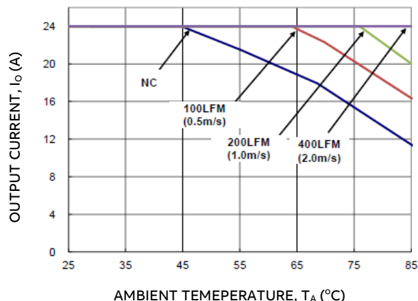
Figure 20. Output Current Derating for the Module with 18H Heatplate; Airflow in the Transverse Direction from V_{out(-)} to V_{out(+)} ; V_{IN} = 24V , V_O = 5V
