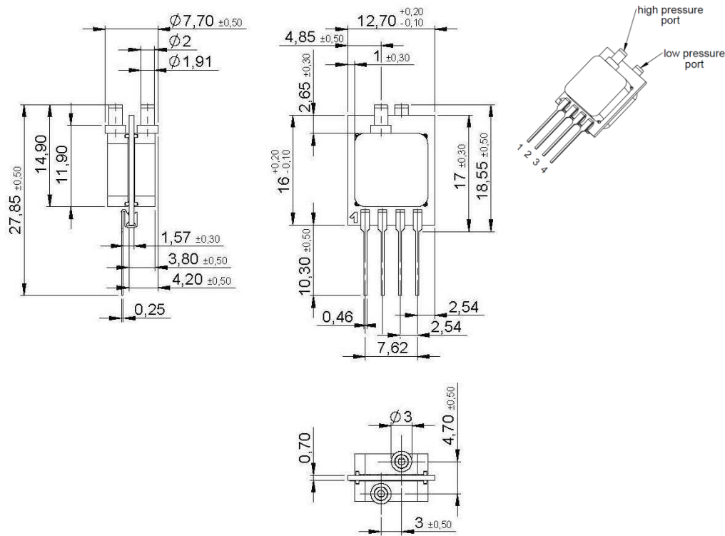
HCLAxxxTxxx (SIL, 2 ports top side)
