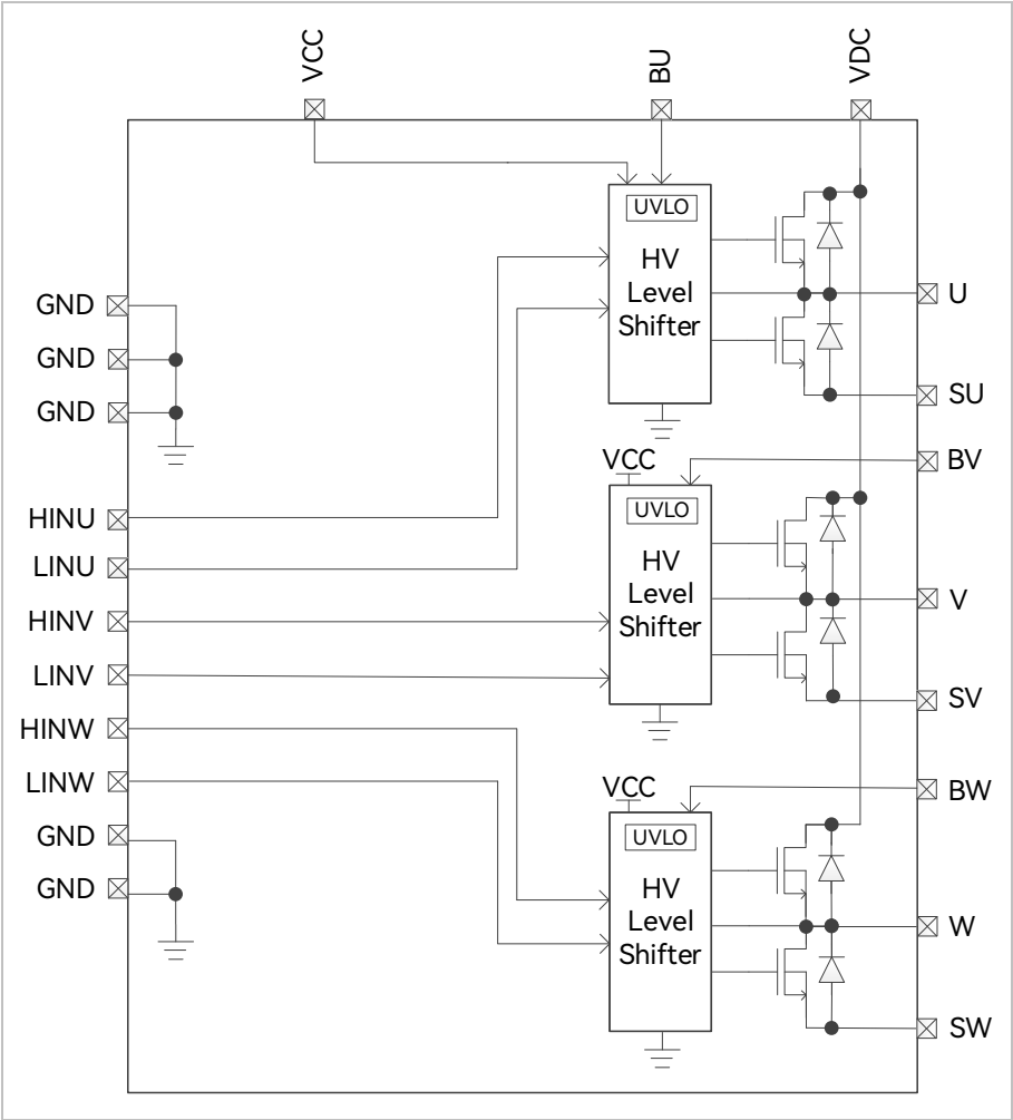
Figure 1-2 Functional Block Diagram of FE0561AAS
