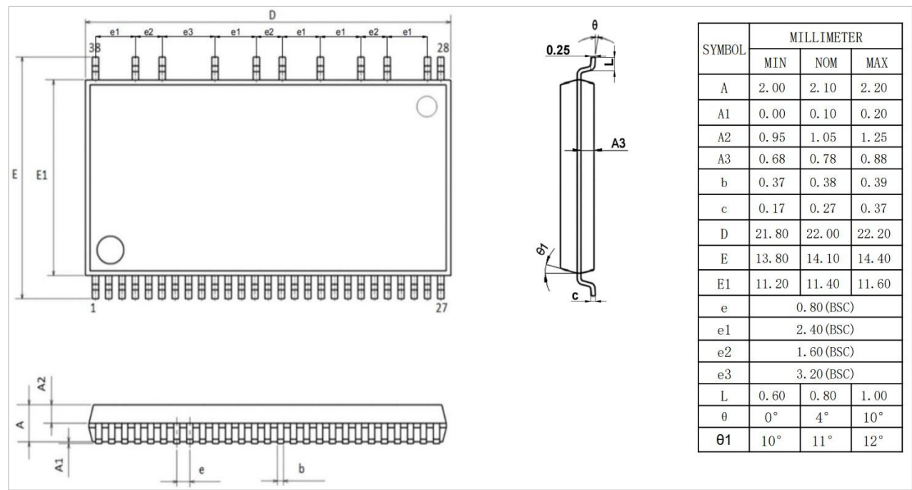
Figure 2-1 FE0561AAS SSOP A54-38 Package Drawings and Dimensions
