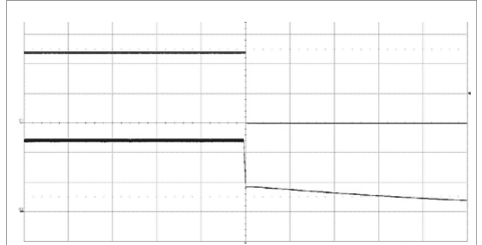
Shut-down enabled by disconnecting V_I at: T_{P1} = +25^\circ\text{C} , V_I = 48\text{ V} , I_O = 2.5\text{ A} resistive load. Top trace: output voltage (5 V/div.). Bottom trace: input voltage (20 V/div.). Time scale: (200 ms/div.).
