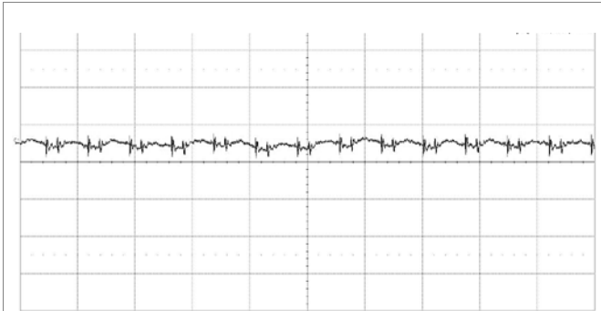
Output voltage ripple at: T_{P1} = +25^{\circ}\text{C} , V_I = 48\text{ V} , I_O = 6\text{ A} resistive load. Trace: output voltage (20 mV/div.). Time scale: (5 μs/div.). 20MHz bandwidth
