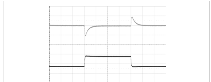
Output disabled by removing V_i at: T_{P1} = +25^\circ\text{C} , V_i = 48\text{ V} , I_o = 1.25\text{ A} electronic load. Top trace: output voltage (5 V/div). Bottom trace: input voltage (20 V/div). Time scale: (1 ms/div).
