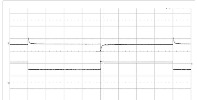
Output voltage response to load current step-change (1.25-1.875-1.25 A) at: T_{P1} = +25^\circ\text{C} , V_I = 48\text{ V} . Top trace: output voltage (500 mV/div.). Bottom trace: load current (1 A/div.). Time scale: (2 ms/div.).
