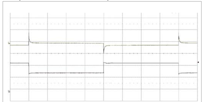
Output voltage response to load current step- change (3.5-5.25-3.5 A) at: T_{P1} = +25^{\circ}\text{C} , V_I = 48\text{ V} . Top trace: output voltage (200 mV/div.). Bottom trace: load current (2 A/div.). Time scale: (2 ms/div.).
