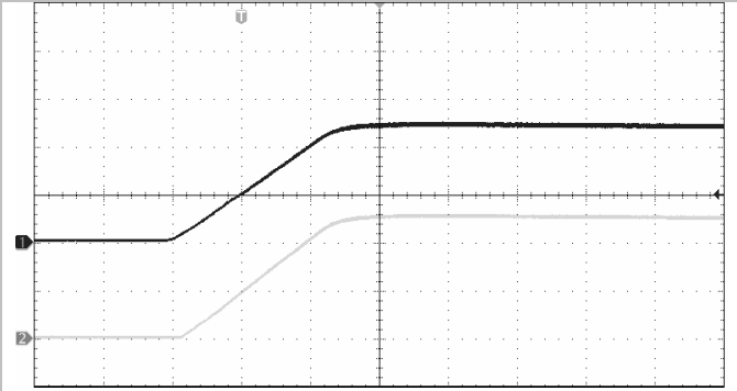
Start-up, enabled by connecting V_i at: T_{P1} = +25^\circ\text{C} , V_i = 24\text{ V} , V_o = 5\text{ V} I_o = 200\text{ mA} resistive load.
