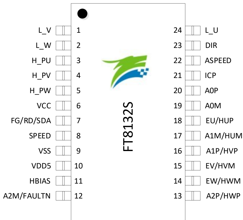
Figure 1-6 FT8132 SSOP24 Pinout Diagram
