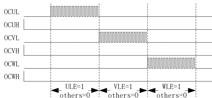
Figure 20-8 Pre-charge Waveform
