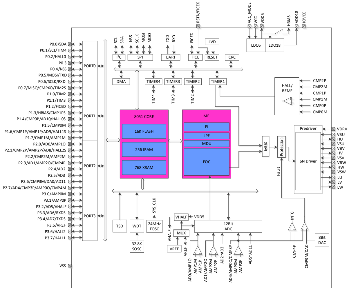
Figure 1-5 Functional Block Diagram of FU6861Q2
