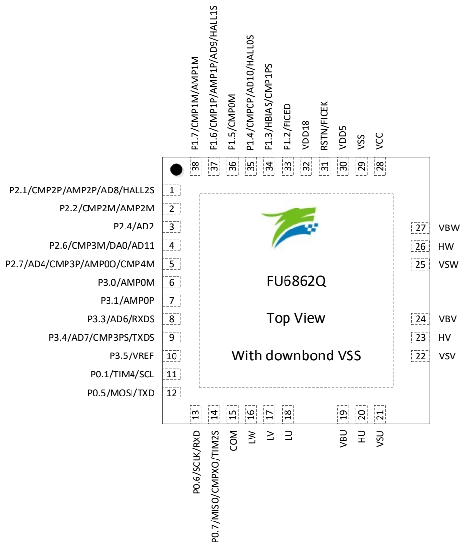
Figure 2-9 FU6862Q QFN48_38 Pinout Diagram
