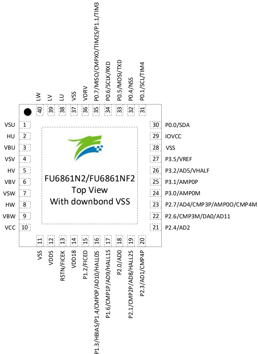
Figure 2-7 FU6861N2/FU6861NF2 QFN40 Pinout Diagram
