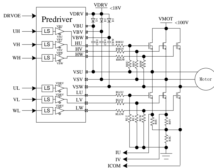
Figure 20-13 Block Diagram of 6N Pre-driver Mode (FU6861Q2/FU6861L2/FU6861N2/FU6861NF2)
