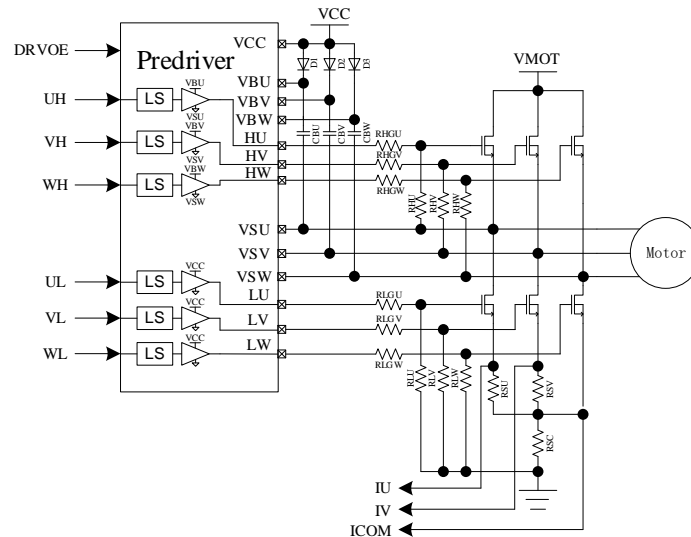
Figure 20-14 Block Diagram of 6N Pre-driver Mode (FU6862L/FU6862Q)
