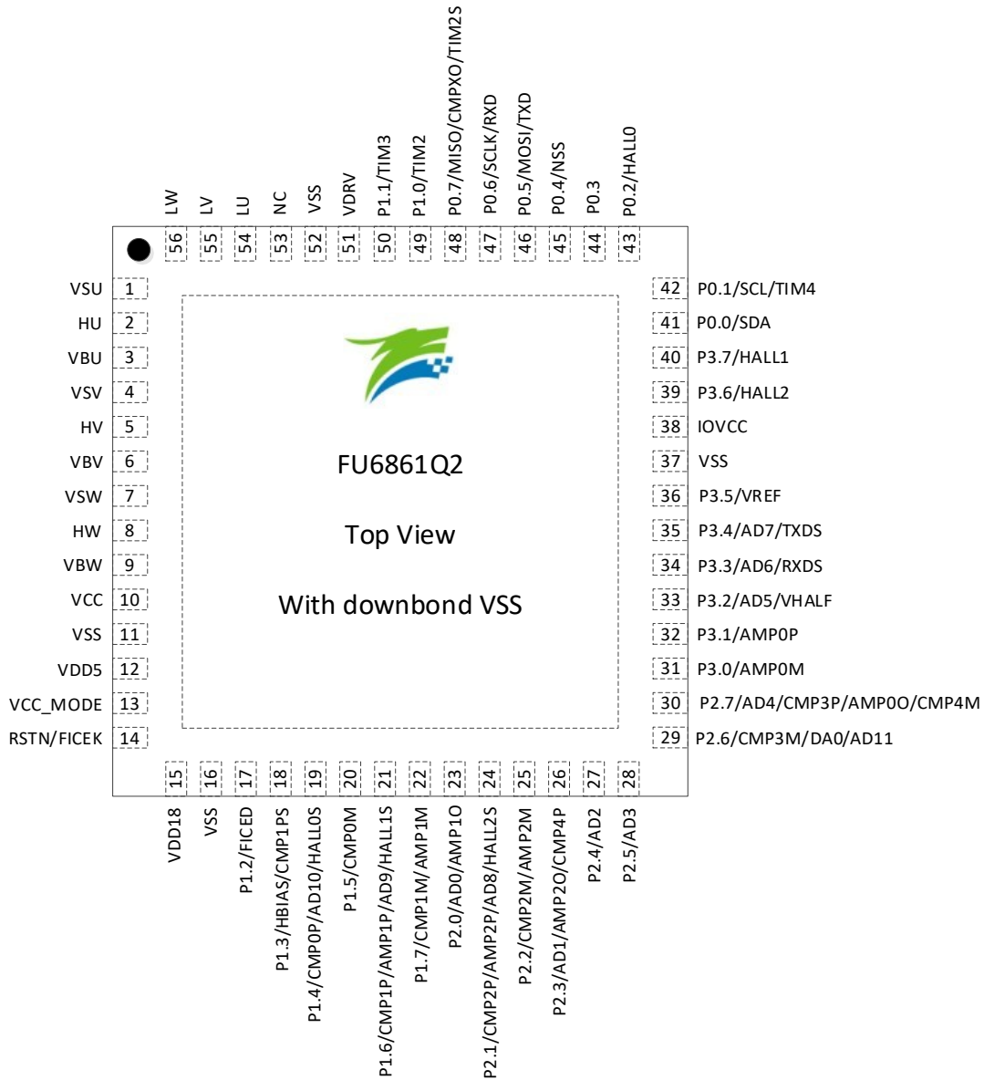
Figure 2-5 FU6861Q2 QFN56 Pinout Diagram
