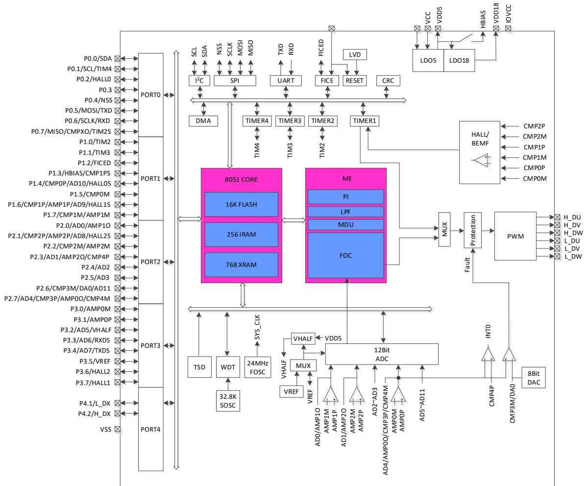
Figure 1-1 Functional Block Diagram of FU6812L2
