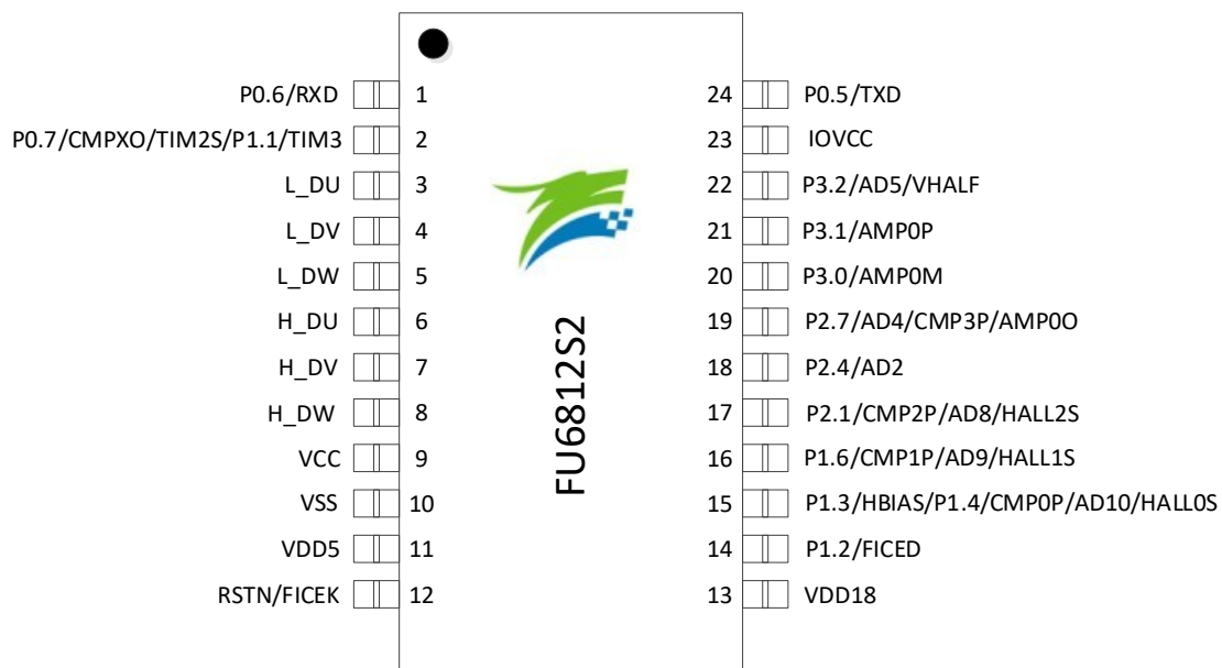
Figure 2-3 FU6812S2 SSOP24 Pinout Diagram
