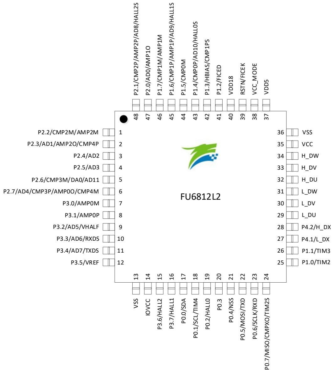
Figure 2-1 FU6812L2 LQFP48 Pinout Diagram
