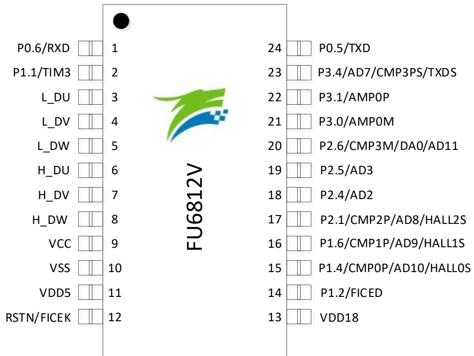
Figure 2-4 FU6812V SSOP24 Pinout Diagram
