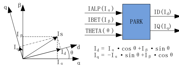
Figure 15-5 Park Transform
