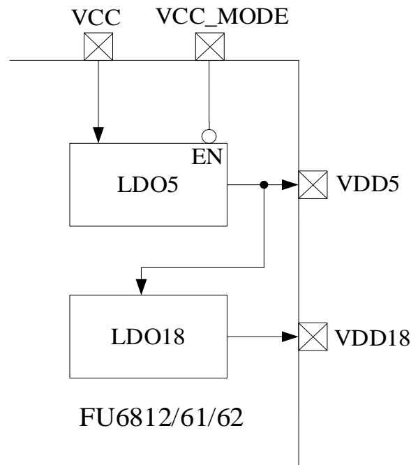
Figure 31-1 Functional Block Diagram of Power Supply
