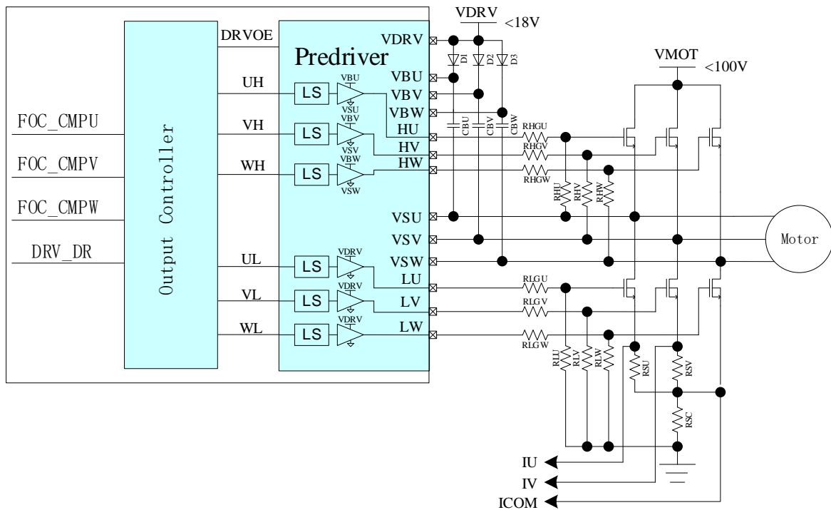
Figure 20-2 Block Diagram of FU6861 Driver Module
