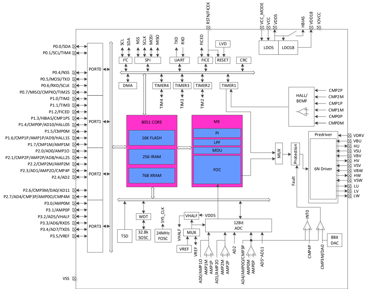
Figure 1-6 Functional Block Diagram of FU6861L2
