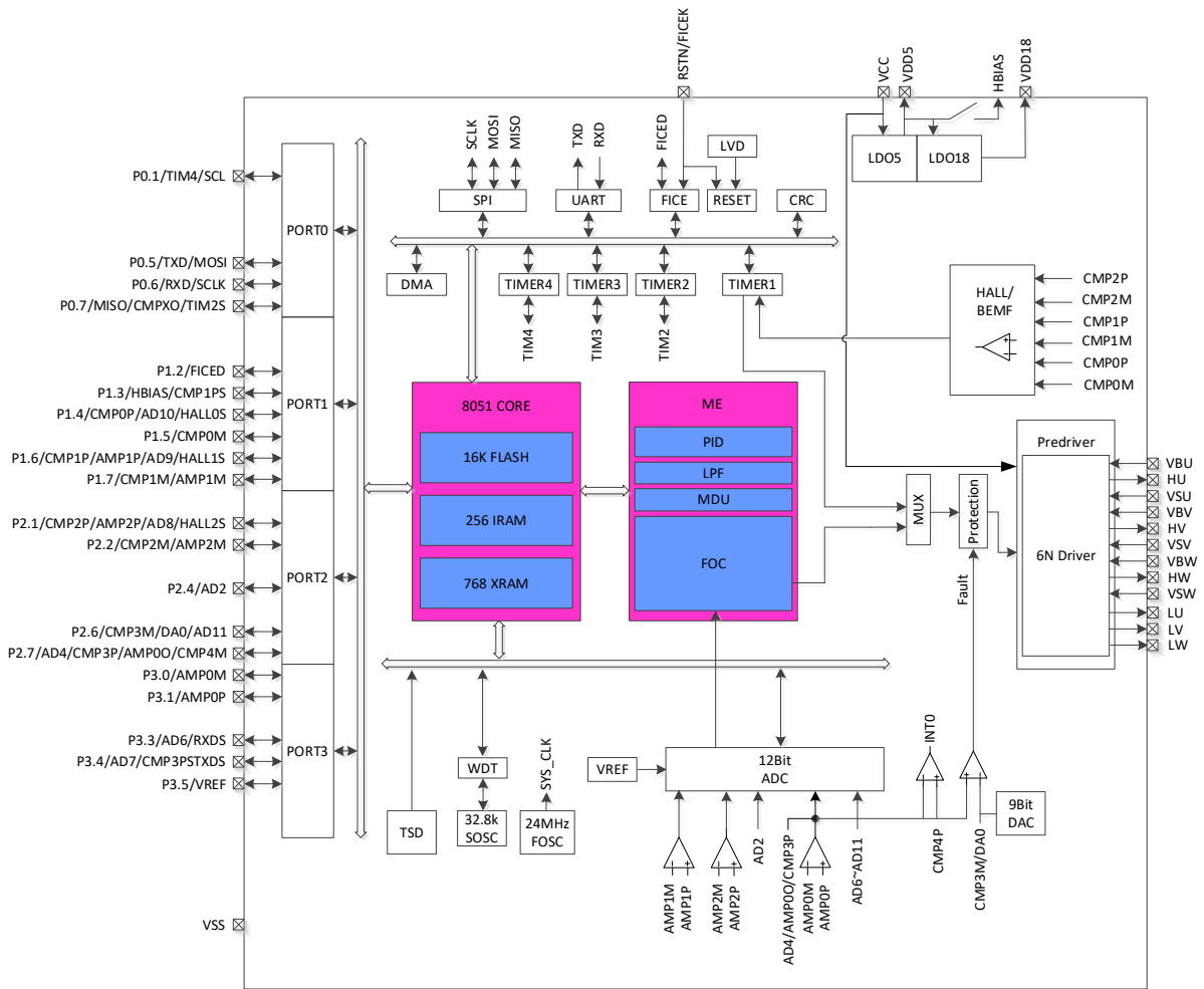
Figure 1-9 Functional Block Diagram of FU6862L/FU6862Q
