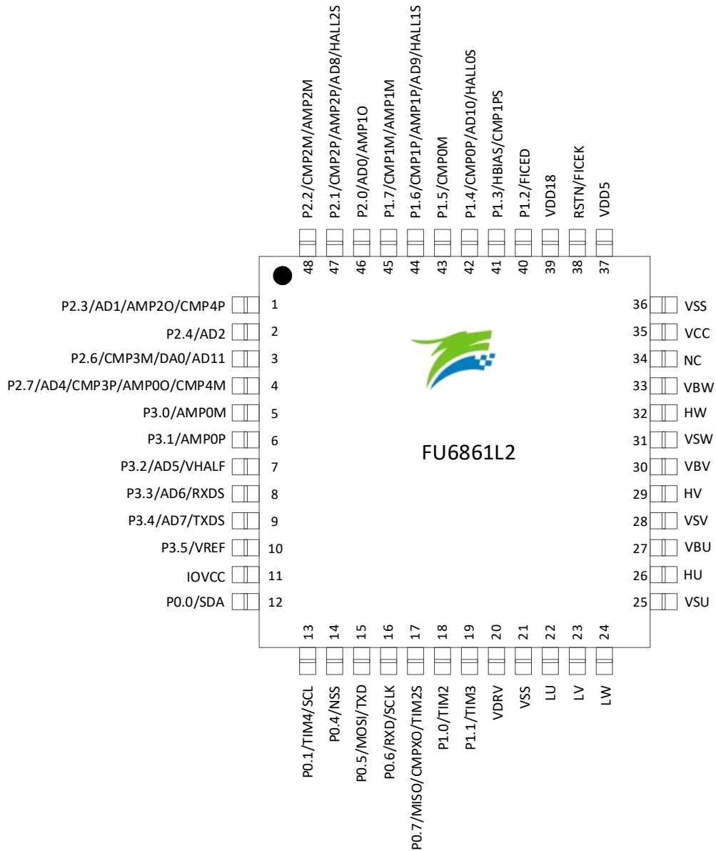
Figure 2-6 FU6861L2 LQFP48 Pinout Diagram
