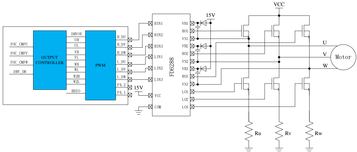
Figure 20-12 Block Diagram of PWM Mode
