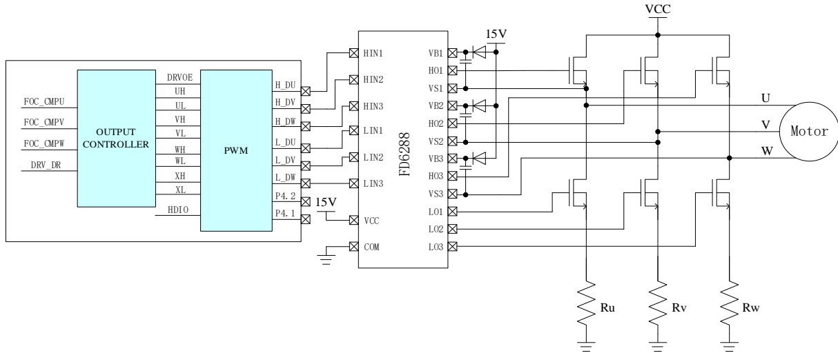
Figure 20-1 Block Diagram of FU6812 Driver Module
