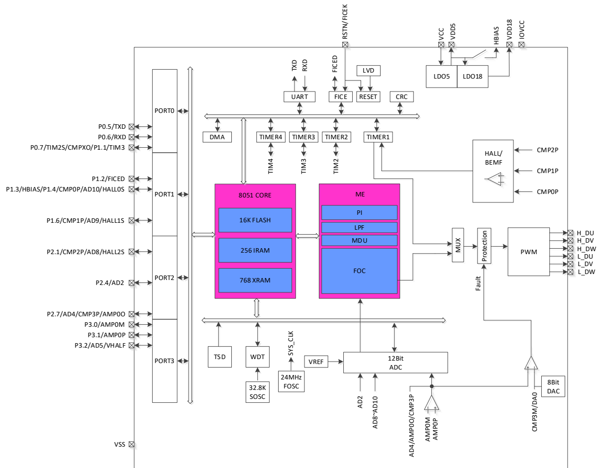
Figure 1-3 Functional Block Diagram of FU6812S2
