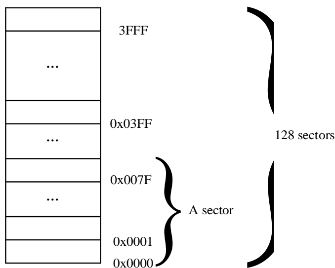
Figure 33-3 ROM Sectors
