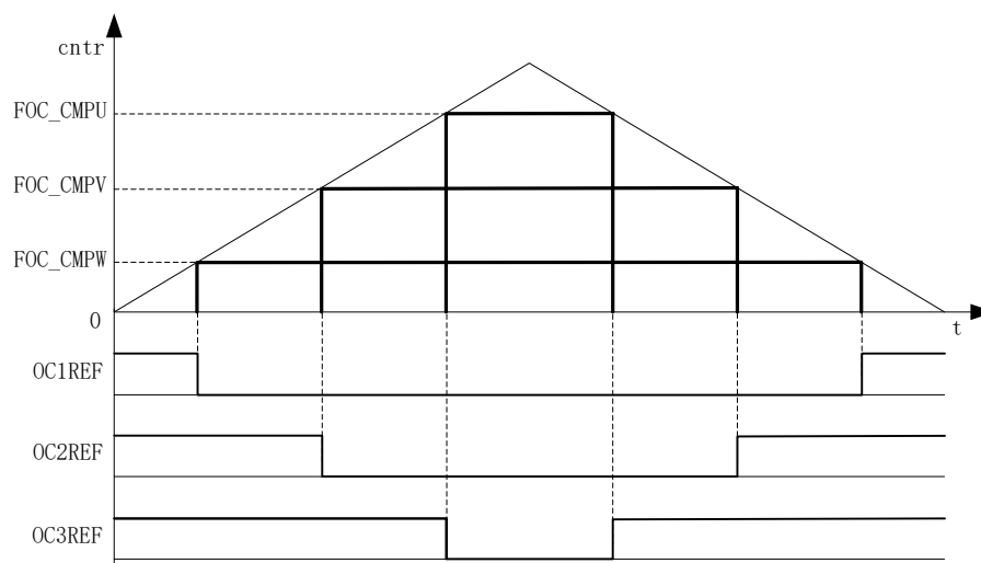
Figure 20-5 PMW Generation
