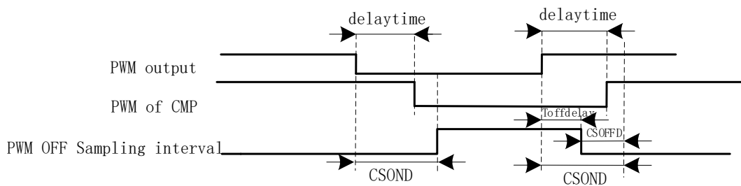
Figure 17-12 PWM OFF Sampling Mode
