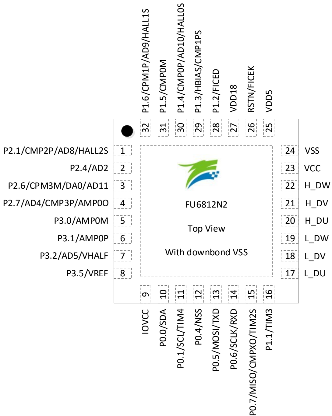
Figure 2-2 FU6812N2 QFN32 Pinout Diagram
