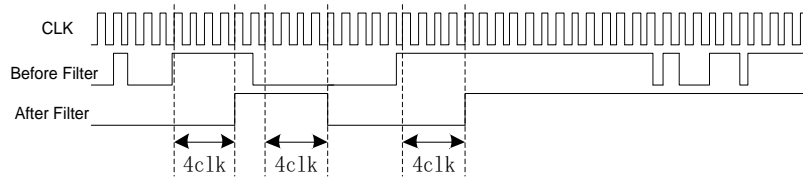
Figure 17-4 Timing Diagram of Filter Module
