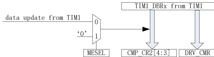
Figure 20-7 Timer1 Automatic Control of DRV_CM and CMP_CR2[4:3]
