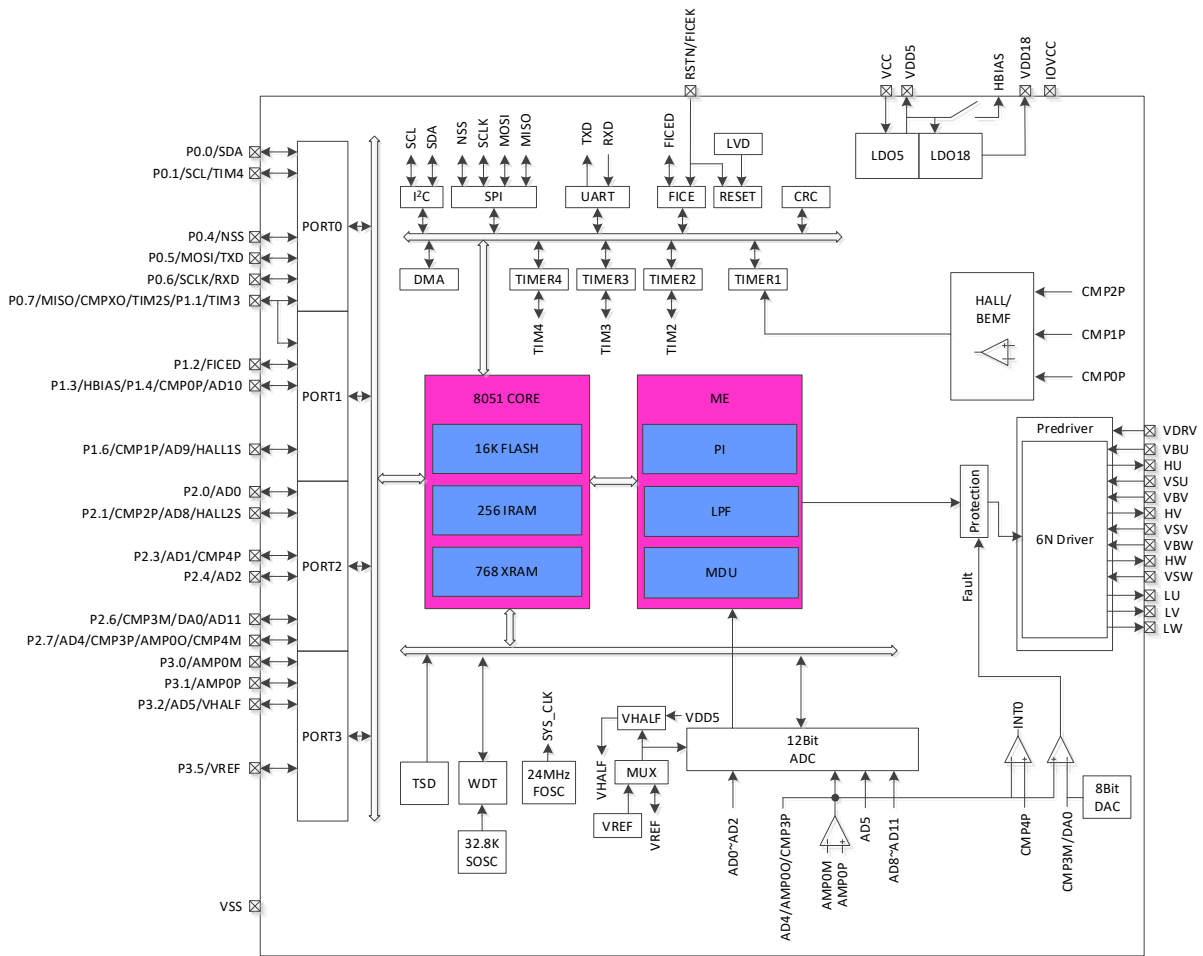
Figure 1-8 Functional Block Diagram of FU6861NF2
