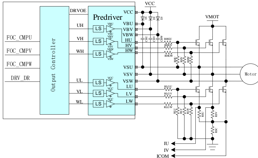
Figure 20-3 Block Diagram of FU6862 Driver Module
