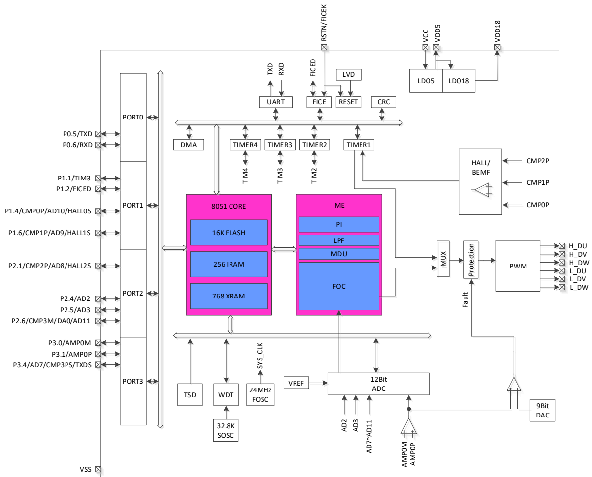
Figure 1-4 Functional Block Diagram of FU6812V
