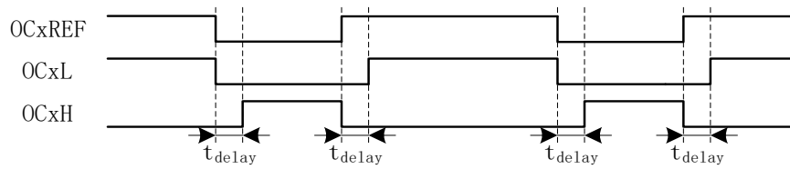
Figure 20-6 Complementary Outputs with Deadtime Insertion
