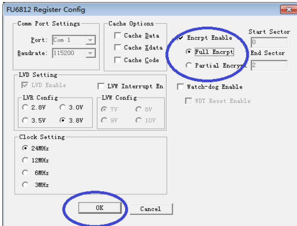
Figure 35-2 Full Code Protection Mode
