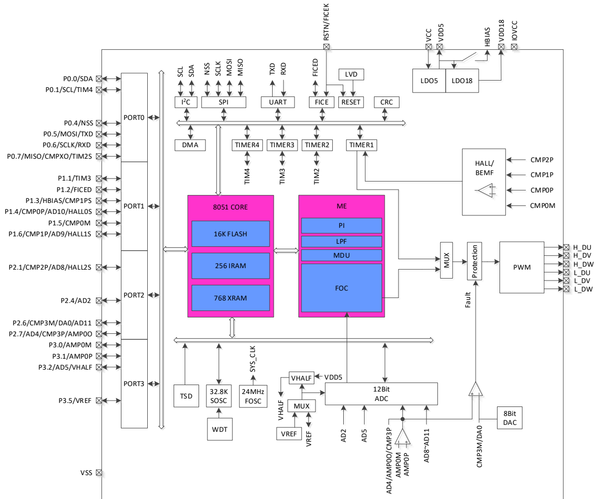
Figure 1-2 Functional Block Diagram of FU6812N2
