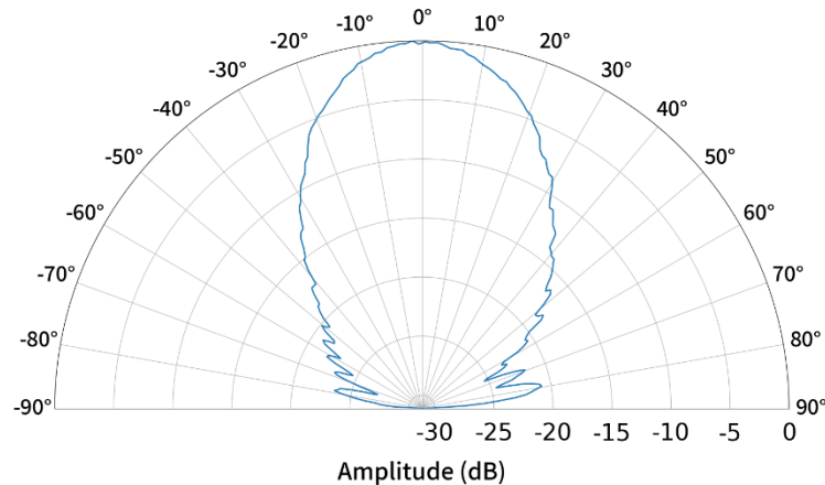
Figure 2. Typical Beam Pattern – MOD-ICU-20201-00-01 45 deg FoV module (Measured with a 1 m 2 flat plate target at a 1m range)
