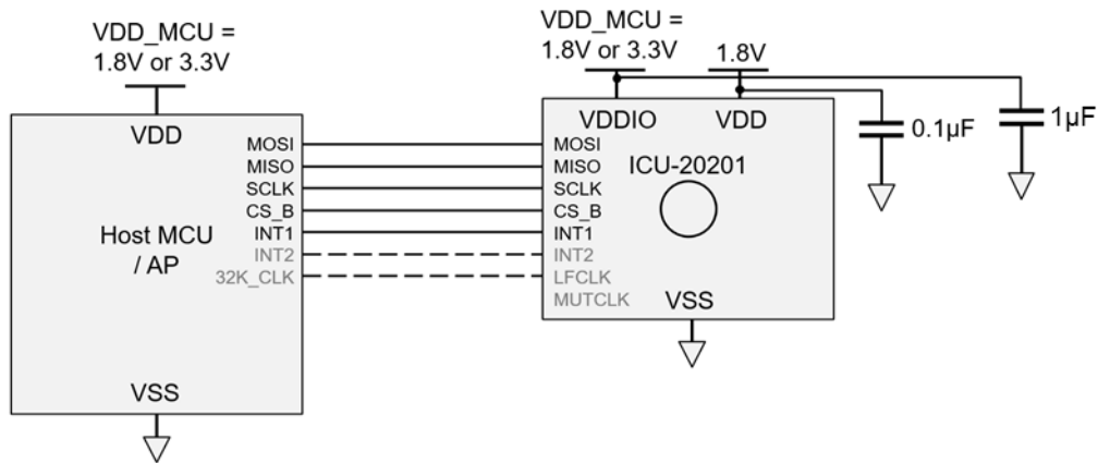
Figure 3. Single Transceiver Operation. Dashed connections are optional. For 3-wire SPI operation, simply short MOSI and MISO near ICU-20201.
