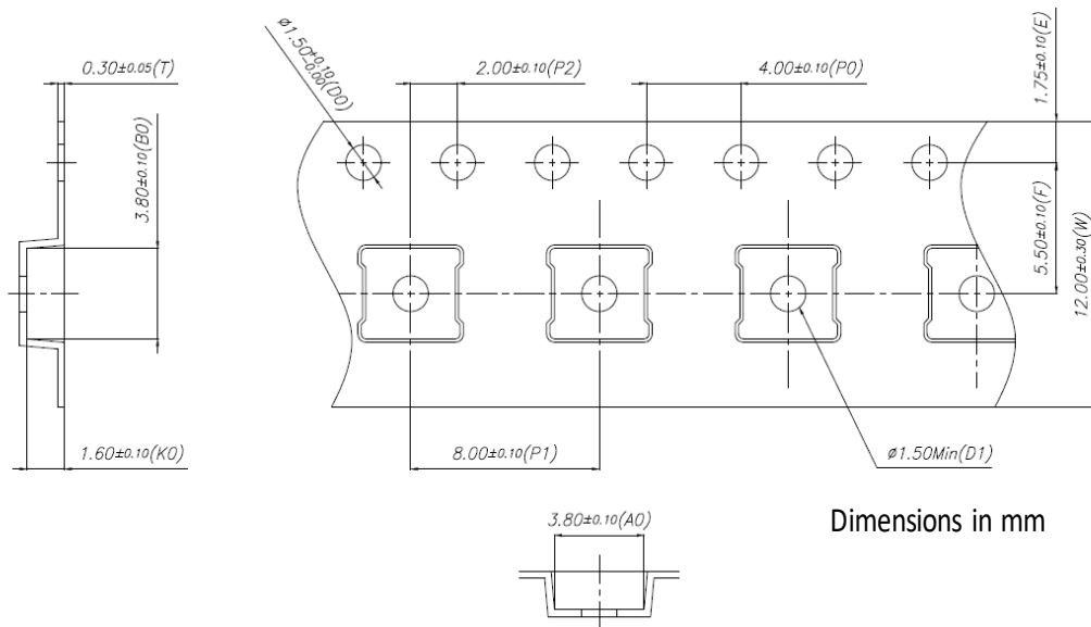
Figure 9. Tape & Reel Specifications
