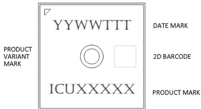
Figure 8. Packaging Marking
