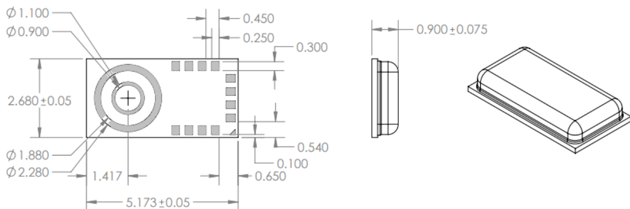
Figure 11. Package dimensions
