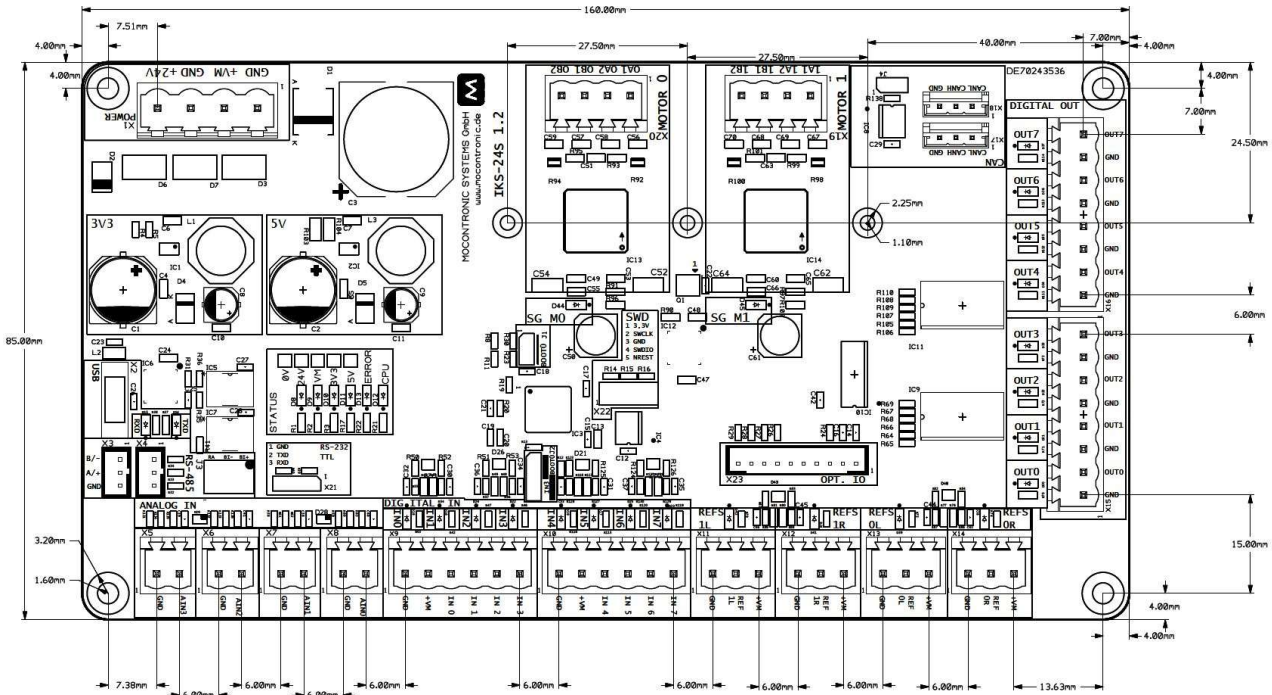
figure 2 dimensions
