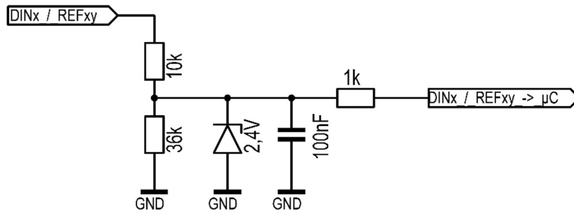
figure 7 circuitry of digital an reference switch inputs
