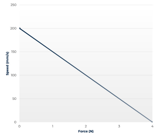
Speed-Force Curve for LBS Series Linear Motor
