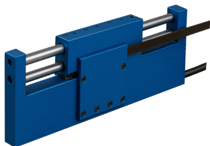
LRMO-150 Series Linear Motor without Encoder
