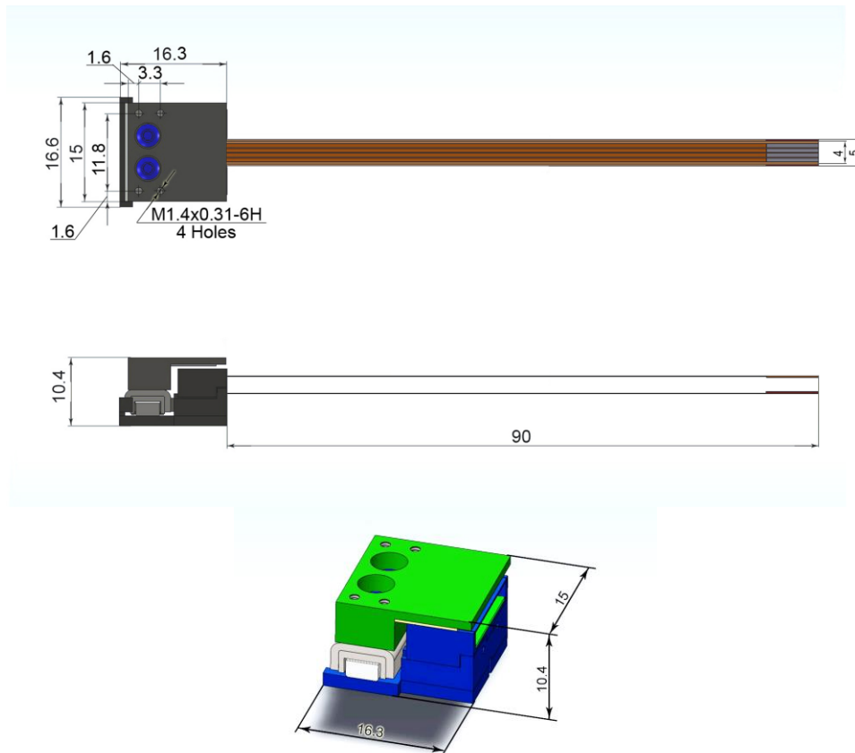
Figure3B. LRMO piezo actuator with factory-fitted encoder. Dimensions (mm)
