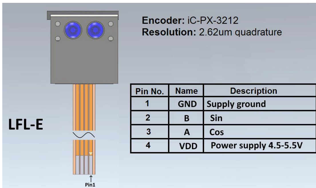
Figure 6 – iC-PX3212 Encoder Pinouts
