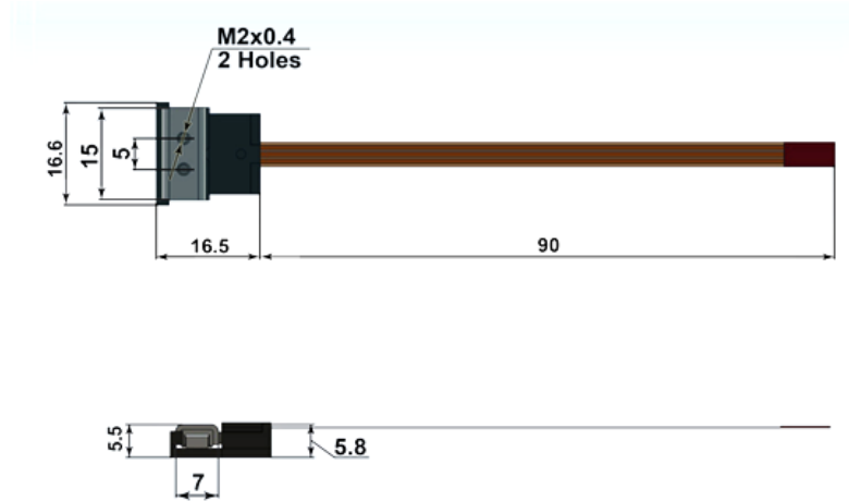
Figure3A. LRMO Linear Piezo actuator without factory-fitted encoder. Dimensions (mm)
