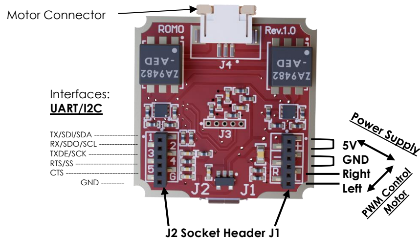
Figure 5. Driver board bottom view
