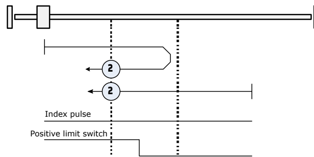
Figure 15: Homing Method 2
