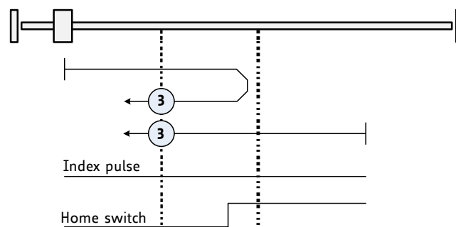
Figure 16: Homing Method 3
