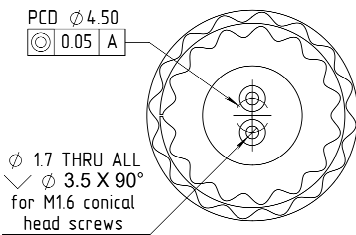
Rotor mounting
