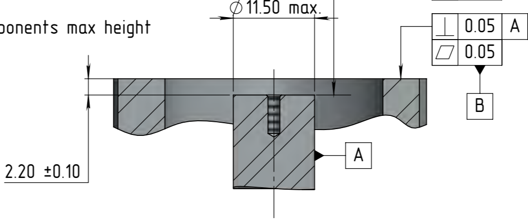
Customer mounting: tolerances and requirements
