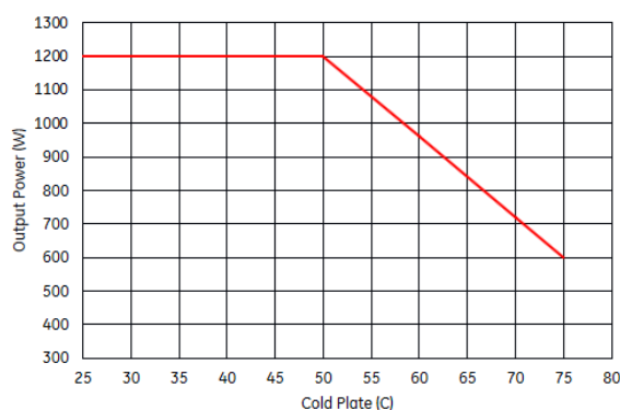
Low line at T_c > 50^\circ\text{C} , 2%/°C
