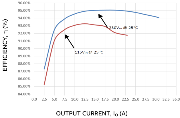
Figure 1. Rectifier Efficiency versus Output Current.
