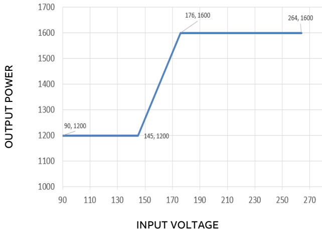
Figure 15. Output power derating below V_{IN} of 185 V AC
