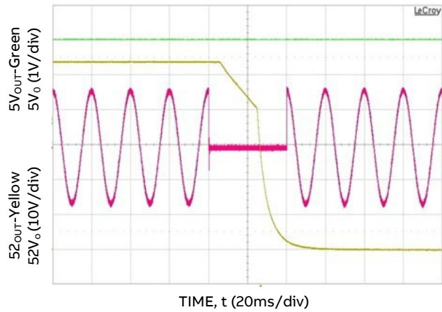
Figure 13. 40ms AC dropout @ full load, V_{IN} = 230V_{AC}
