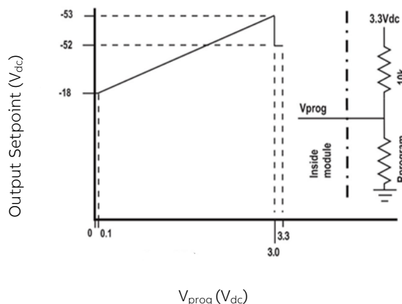
Factory default setting driven by V_{\text{prog}}
