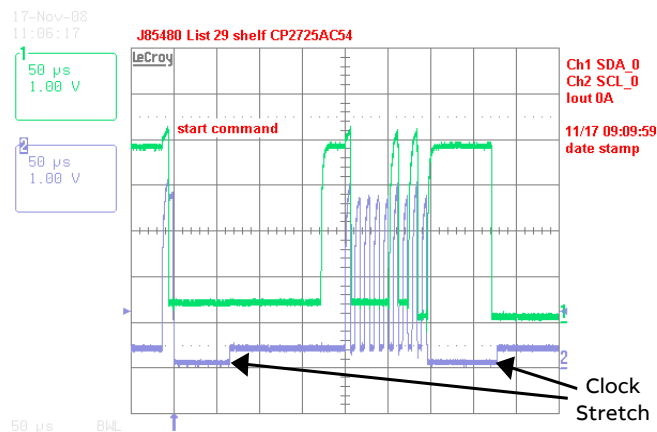
Figure 13. Example waveforms showing clock stretching.
