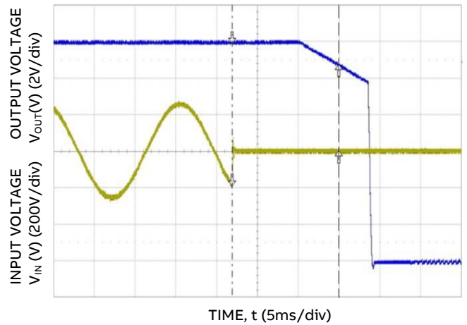
Figure 10. Hold-up ( V_{IN} = 230V , I_o = 80\% I_{o,max} ).
