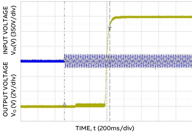
Figure 7. Start-up ( V_{IN} = 90V , I_o = I_{o,max} ).
