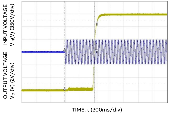
Figure 8. Start-up ( V_{IN} = 264V , I_o = I_{o,max} ).
