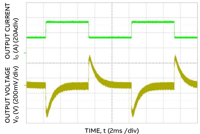
Figure 12. Transient Response to Dynamic Load Change from 50% to 100% I_{o,max} at V_{IN} = 230V .
