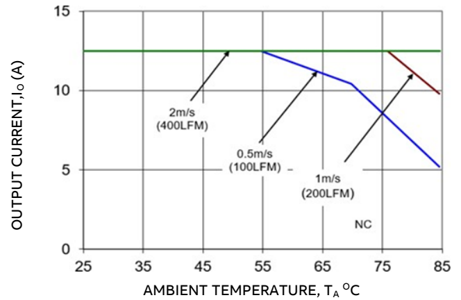
Figure 2. Derating Output Current versus Ambient Temperature and Airflow. Data shown for 115V AC in, at 230V AC in derating is the same or better. For derating at other input voltages, consult the ABB Technical representative.
