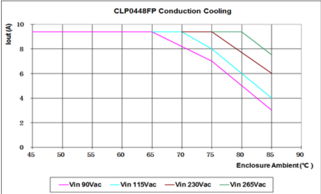
Z01 Derating Curves (Enclosure Application)
