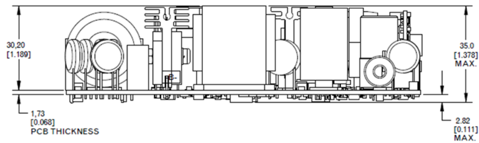
SIDE VIEW
