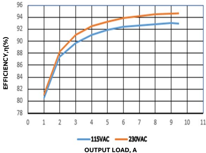
Figure 1: Power Supply Efficiency Versus Output Current
