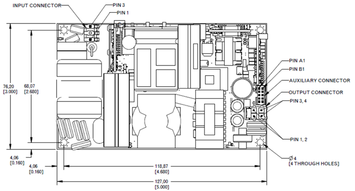
TOP VIEW
