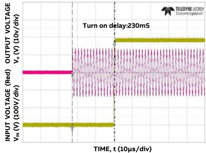
Figure 4. Typical Start-up ( V_{IN} = 90V_{ac} , Full Load)
