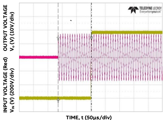
Figure 5. Typical Start-up ( V_{IN} = 230V , Full Load)
