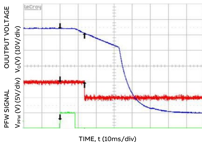
Figure 12. PFW alarmed 19.6ms prior to V_o < 40V , output load: 38A, V_{IN} = 185V_{AC} .
