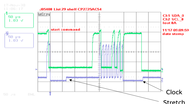
Figure 14. Example waveforms showing clock stretching.
