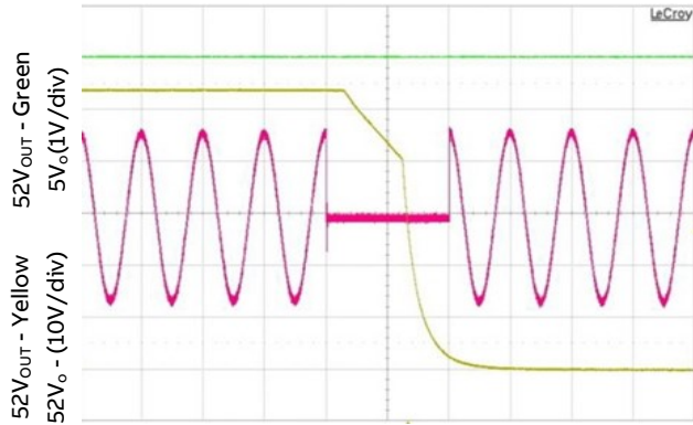
TIME, t (20ms/div) Figure 13. 40ms AC dropout @ full load, V_{IN} = 230V_{AC}
