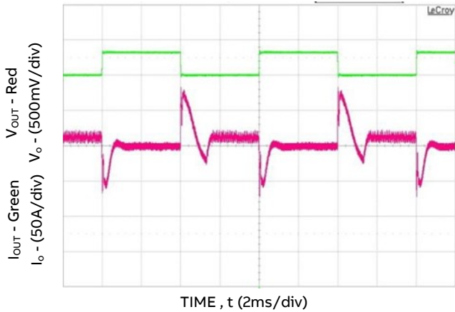
Figure 7. Transient response 52V DC load step 10 – 60%, Slew rate: 1A/μs, V IN = 230V AC
