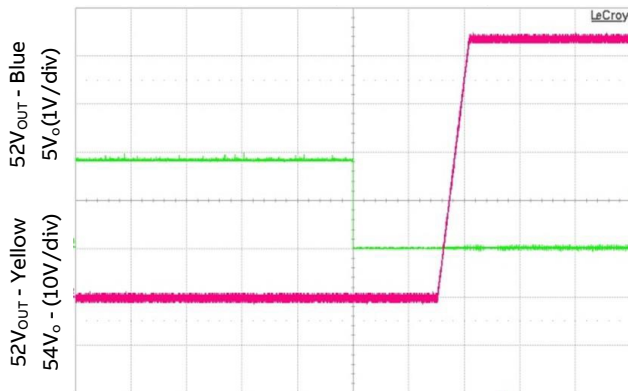
TIME, t (500ms/div) Figure 15. Turn-OFF at full load, V_{IN}=230V_{AC}
