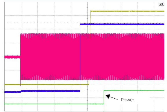
TIME, t (1s/div) Figure 14. Turn-ON at full load V_{IN} = 230V_{AC} .
