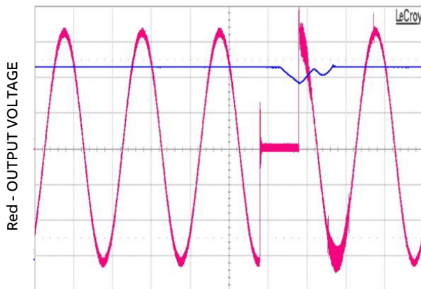
TIME, t (100ms/div) Figure 17. Time delay from sending the I 2 C command and executing the output voltage change.
