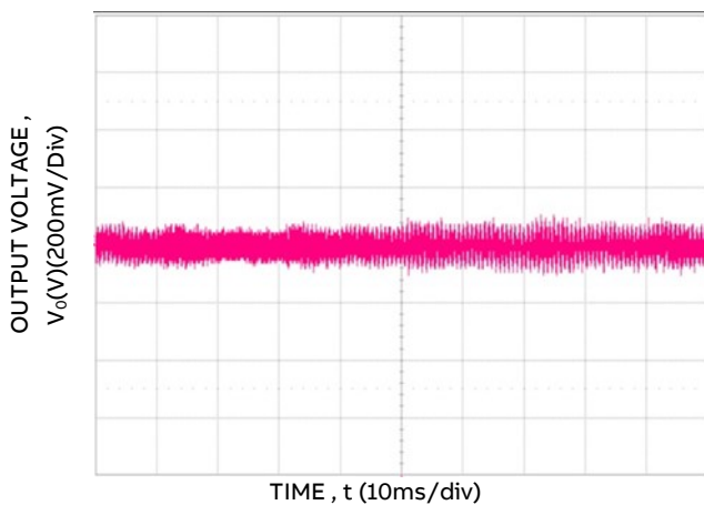
Figure 5. 52V dc output ripple and noise, full load, V_{IN} = 185V_{AC} , 20MHz bandwidth
