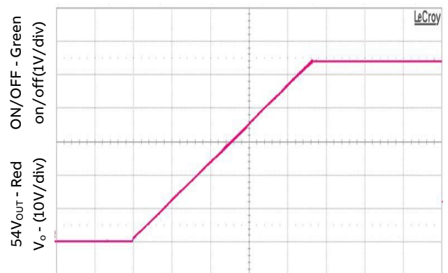
TIME, t (200ms/div) Figure 16. 52V dc turn-OFF delay when ON/OFF is di-asserted, V_{IN}=230V_{AC} - i 2 C mode.
