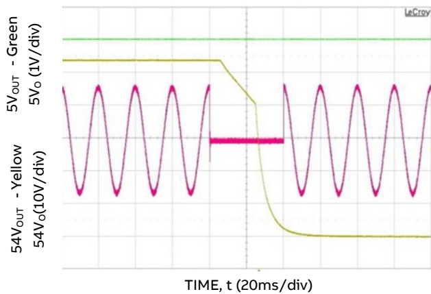
Figure 13. 40ms AC dropout @ full load, V_{IN} = 230V_{AC} .
