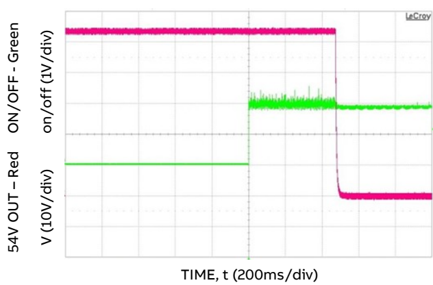
Figure 16. 54V DC turn-OFF delay when ON/OFF is di-asserted, V_{IN}=230V_{AC} - I 2 C mode.
