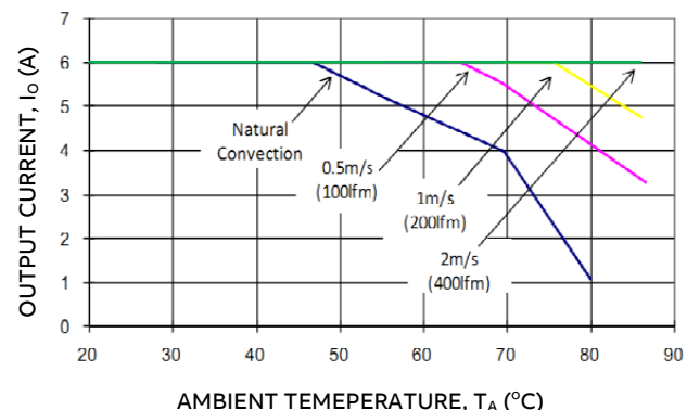
Figure 18. Output Current Derating for the Module with -18 Heatplate; Airflow in the Transverse Direction from V_{out(-)} to V_{out(+)} ; V_{IN} = 24V .
