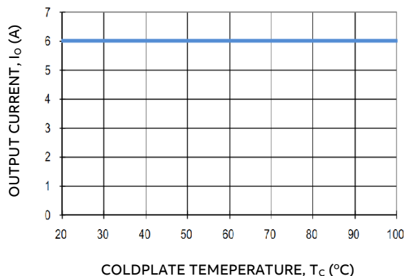
Figure 20. Derated Output Current versus Cold Wall Temperature with local ambient temperature around module at 85°C; V_N = 24V or 48V.
