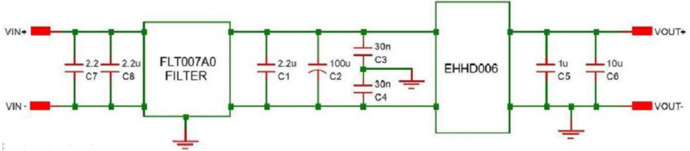
Figure 25. EMC Considerations
