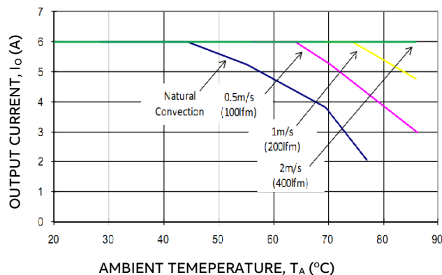
Figure 17. Output Current Derating for the Open Frame Module; Airflow in the Transverse Direction from V_{out(-)} to V_{out(+)} ; V_{IN} = 24V
