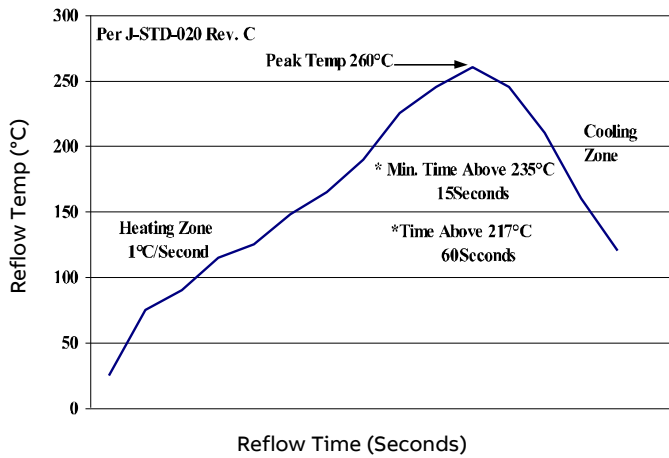
Figure 26. Recommended linear reflow profile using Sn/Ag/Cu solder.
