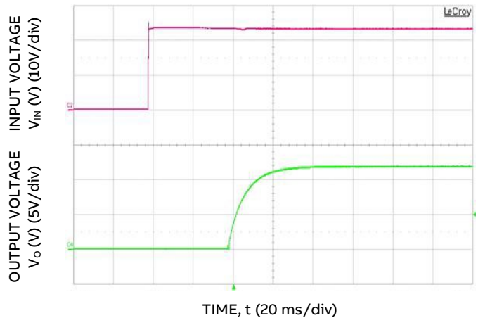
Figure 6. Typical Start-up Using Input Voltage ( V_{IN} = 24\text{ V} , I_o = I_{o,max} ).
