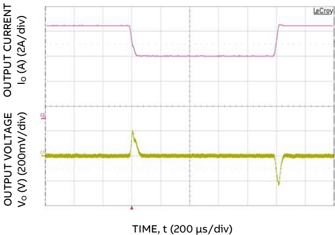
Figure 3. Transient Response to 0.1A/μS Dynamic Load Change from 50% to 75% to 50% of full load, V_{in} = 24\text{ V}
