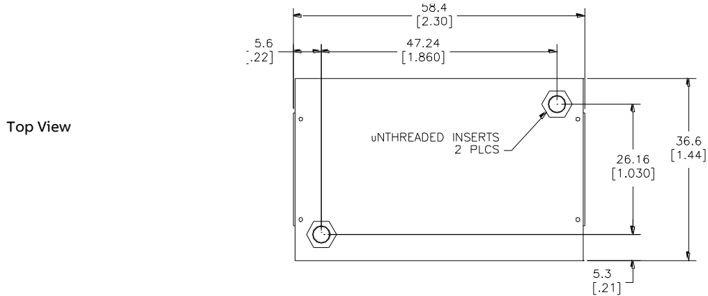
Mechanical Outline for EHHD_120W Through-Hole Module with 1/4th Brick Heat Plate
