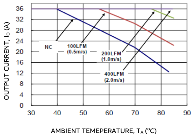
Figure 19. Output Current Derating for the Module with Heatplate; Airflow in the Transverse Direction from V_{out(-)} to V_{out(+)} ; V_{IN}=24V , V_O=3.3V .
