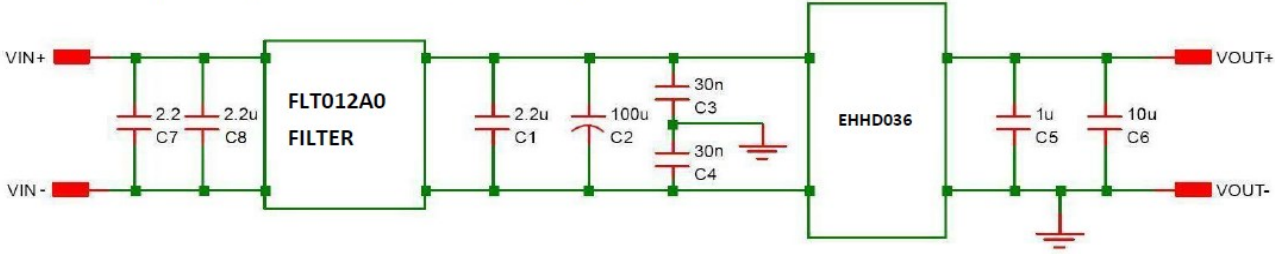
Figure 27. EMC Considerations
