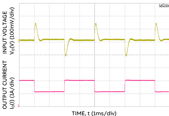
Figure 3. Dynamic Load Change Transient Response from 25% to 50% to 25% of Full Load at Room Temperature and 48V_{in} , 0.1\mu\text{s} , C_{o,ext} = 220\mu\text{F} .
