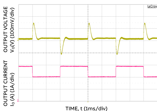
Figure 6. Dynamic Load Change Transient Response from 50% to 75% to 50% of Full Load at Room Temperature and 48V_{in} ; 0.1\mu\text{s} , C_{o,ext} = 220\mu\text{F} .
