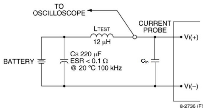
Figure 7. Input Reflected Ripple Current Test Setup.
