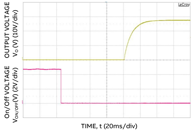
Figure 4. Typical Start-Up Using Remote On/Off; C_{o,ext} = 220\mu\text{F}
