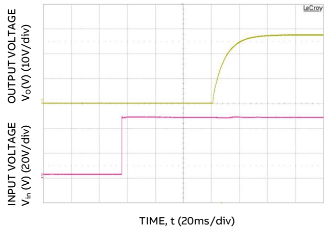
Figure 5. Typical Start-Up from V_{in} , on/off enabled prior to V_{in} step; C_{o,ext} = 220\mu\text{F} .
