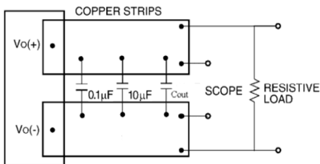
Figure 8. Output Ripple and Noise Test Setup.
