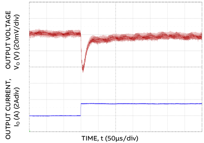
Figure 22. Transient Response to Dynamic Load Change from 5% to 100% at 12 Vin, C out -2x 100μF, C tune - 1.5nF, R tune - 500
