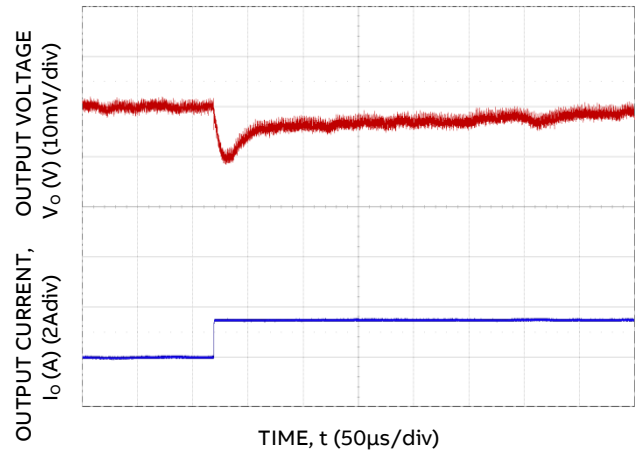
Figure 4. Transient Response to Dynamic Load Change from 5% to 100% at 12 Vin, C out - 2x 330µF, 6x 100µF, C tune - 10µF, R tune - 500 Ω, V IN = 5V.
