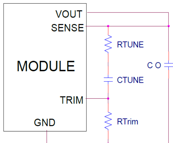
Figure. 45. Circuit diagram showing connection of R_{TUNE}
