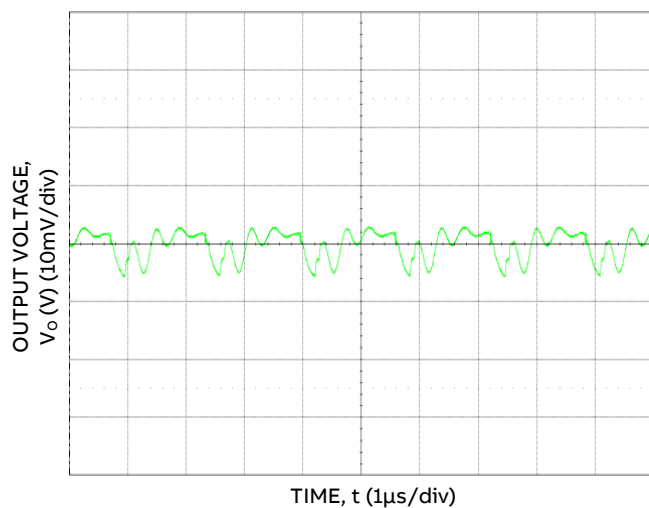
Figure 15. Typical Output Ripple and Noise, (C o = 88 μF Ceramic, V IN = 12 V, I o = I o, max .)
