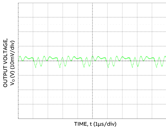
Figure 9. Typical Output Ripple and Noise, (C o = 88 μF Ceramic, V IN = 12 V, I o = I o, max .)
