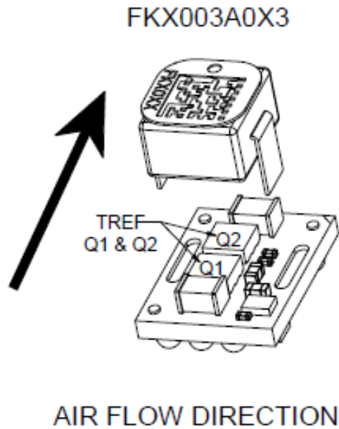
Figure 47. Preferred airflow direction and location of hotspots of the module ( T_{ref} ).
