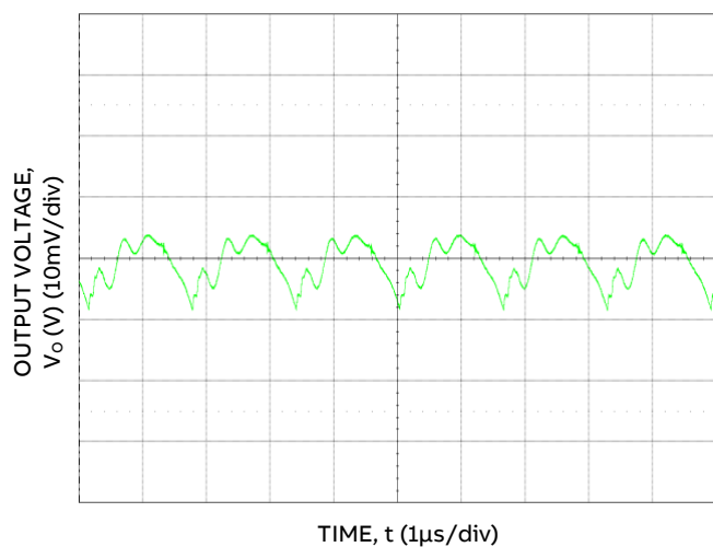
Figure 27. Typical Output Ripple and Noise, (C o = 88 μF Ceramic, V IN = 12 V, I o = I o, max .)
