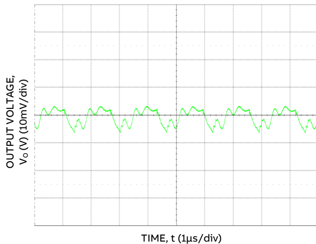
Figure 21. Typical Output Ripple and Noise, (C o = 88 μF Ceramic, V IN = 12 V, I o = I o, max .)
