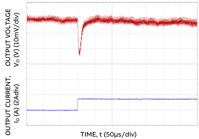
Figure 16. Transient Response to Dynamic Load Change from 5% to 100% at 12 V in , C out - 4x 100μF, C tune - 4.7nF, R tune - 400
