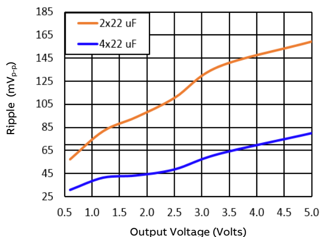
Figure 34. Input ripple voltage for various output voltages with 2x22 µF or 4x22 µF ceramic capacitors at the input (3A load). Input voltage is 12V.
