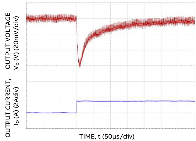
Figure 28. Transient Response to Dynamic Load Change from 5% to 100% at 12 Vin, C out –2x 100μF, C tune - 1nF, R tune – 500
