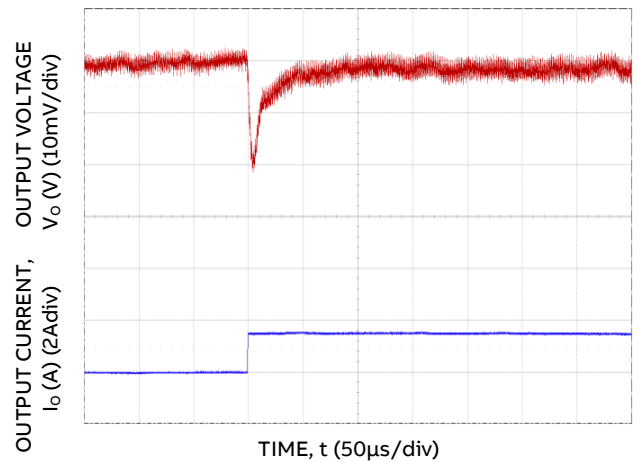
Figure 10. Transient Response to Dynamic Load Change from 5% to 100% at 12 Vin, C out - 4x 100μF, C tune - 4.7μF, R tune - 400
