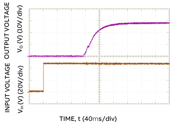
Figure 5. Typical Start-Up from V in,on/off enabled prior to V in step; C o,ext = 470μF.
