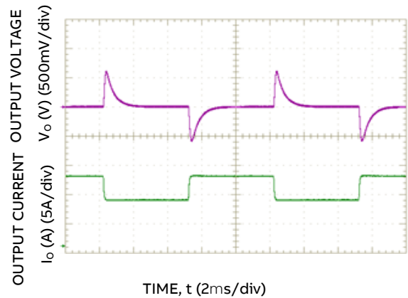
Figure 6. Dynamic Load Change Transient Response from 50% to 75% to 50% of Full Load at Room Temperature and 48V in ; 0.1A/μs, C o,ext = 440μF.
