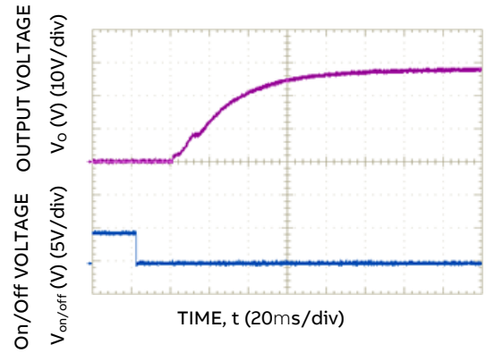
Figure 4. Typical Start-Up Using negative Remote On/Off; C o,ext = 440μF.
