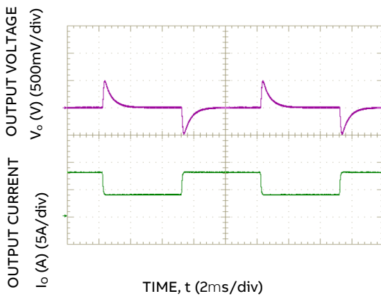
Figure 3. Dynamic Load Change Transient Response from 25% to 50% to 25% of Full Load at Room Temperature and 48V in ; 0.1A/μs, C o,ext = 440μF.
