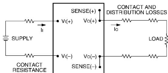
Figure 9. Output Voltage and Efficiency Test Setup.
