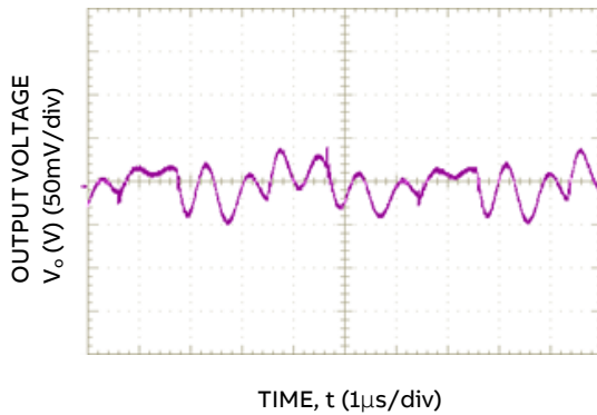
Figure 2. Typical output ripple and Noise at Room Temperature and 48V in ; I o = I o,max ; C o,ext = 440μF.
