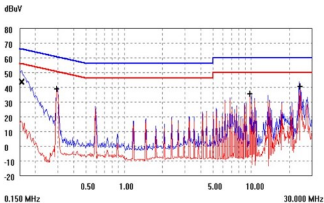
Figure 18. V_{in+} Line EMC signature using above filter, V_{in}=48V , Blue=Quasi Peak, Red=Average.
