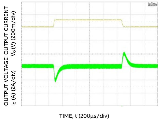
Figure 4. Transient Response to 0.1A/ \mu S Dynamic Load Change from 50% to 75% to 50% of full load, V_{in}=48V , C_o > 100\mu F
