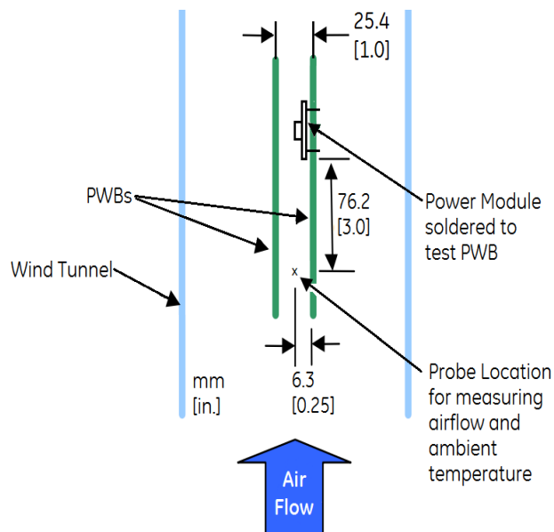
Figure 13. Thermal Test Setup .
