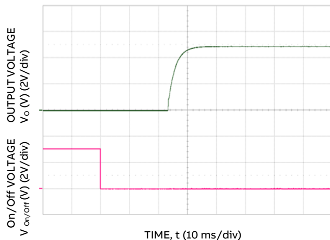
Figure 5. Typical Start-up Using Remote On/Off, negative logic version shown ( V_{IN} = 24 to 48V, I_o = I_{o, max} ).
