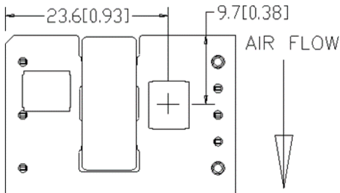
Figure 16. T_{ref} Temperature Measurement Location.
