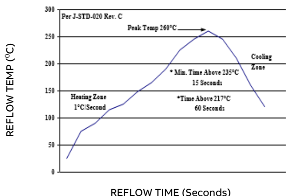
Figure 22. Recommended linear reflow profile using Sn/Ag/Cu solder
