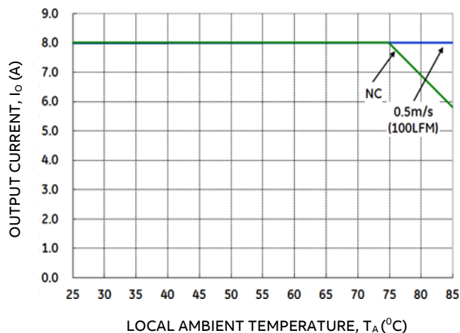
Figure 14. Output Current Derating for the Open Frame KHHD010A0A in the Transverse Orientation; Airflow Direction from Vin(+) to Vin(-); Vin = 24V.
