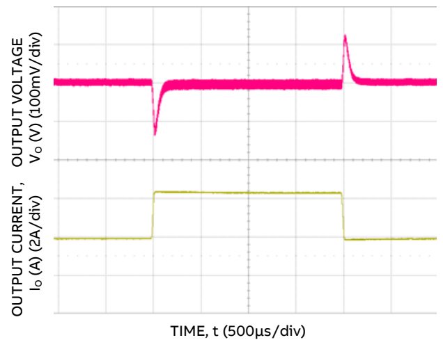
Figure 4. Transient Response to 0.1A/ \mu s Dynamic load Change from 50% to 75% to 50% of full load, V_{in}=48V
