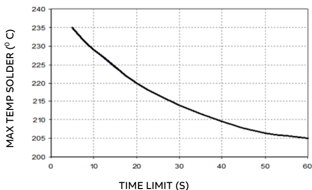
Figure 21. Time Limit, T_{lim} , Curve Above 205 °C Reflow .
