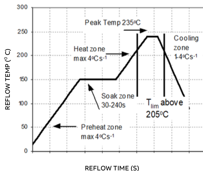
Figure 20. Recommended Reflow Profile for Sn/Pb solder.
