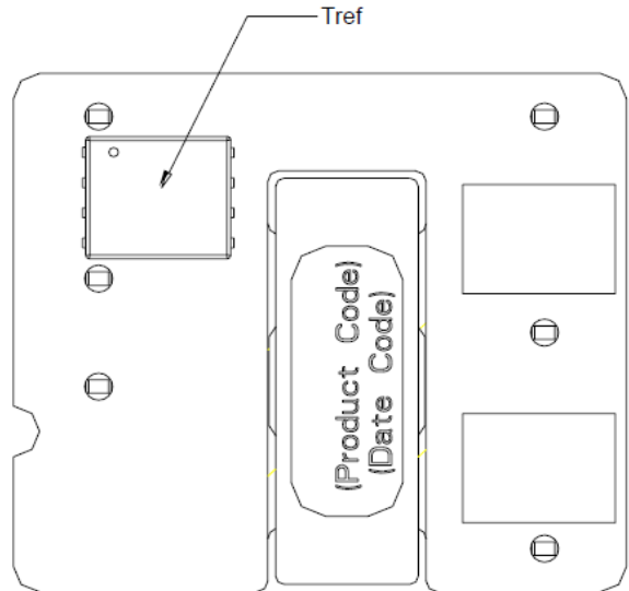
Figure 16. T_{ref} Temperature Measurement Location.
