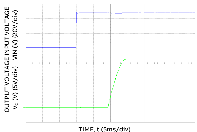
Figure 6. Typical Start-up w/o-P version Using Input Voltage (VIN = 48V, I_o = I_o, max).
