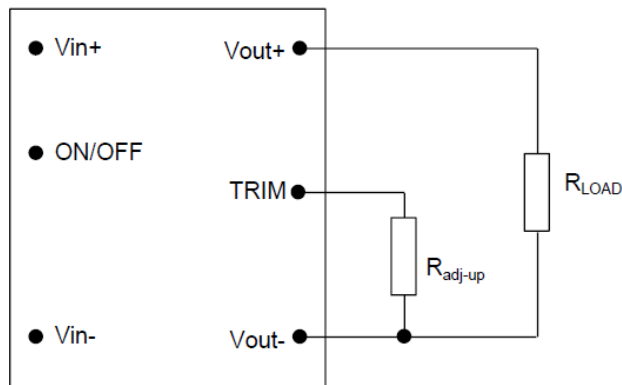
Figure 12. Circuit Configuration to Increase Output Voltage.
